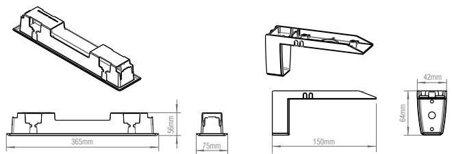
Recess Accessory 108751
