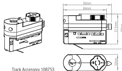
Track Accessory 108753
